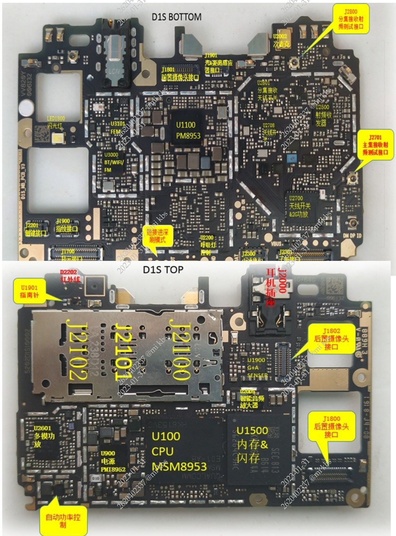
2.2 Red rice6 Pro Distribution map of sub-board components
